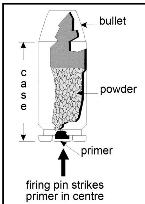
Figure 95. Centre-fire Cartridge
