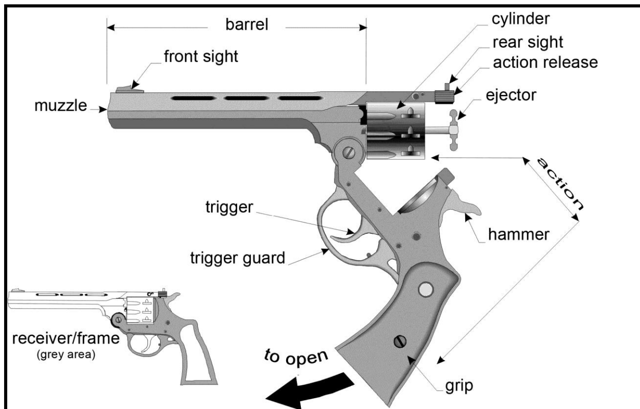
Figure 112. Top-break Revolver
