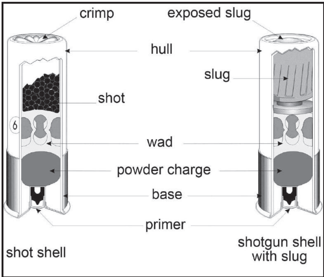
Figure 32. Shotgun Shells
