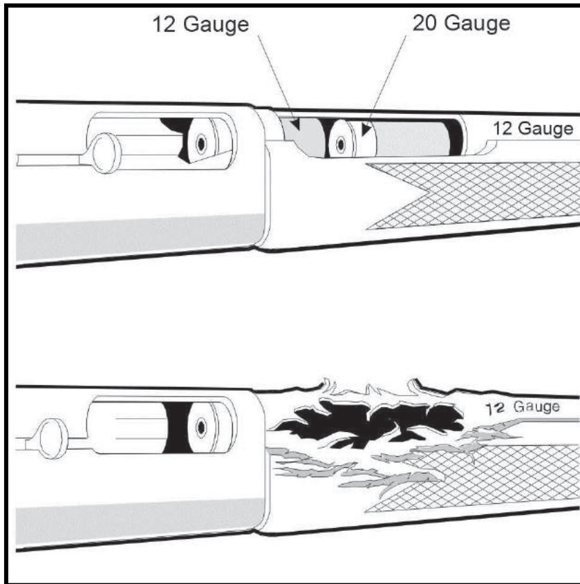
Figure 36. Exploded Chamber
