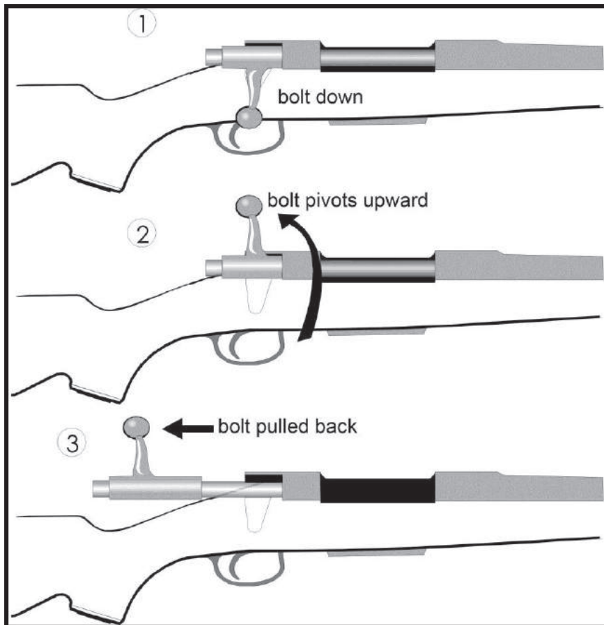
Figure 52. Bolt-action Repeater
