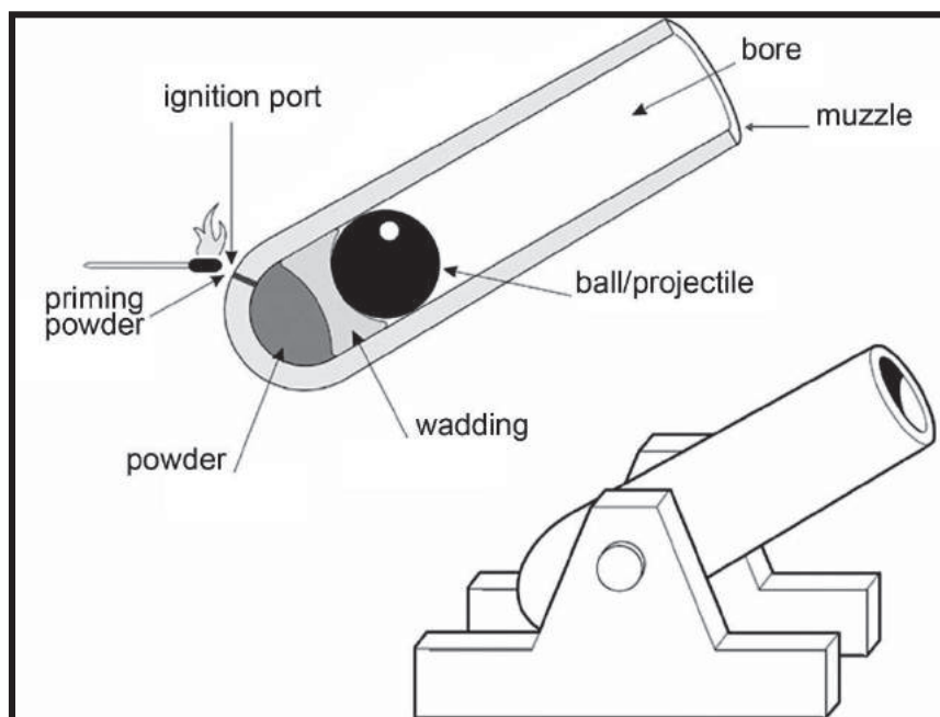
Figure 1. Cannon
