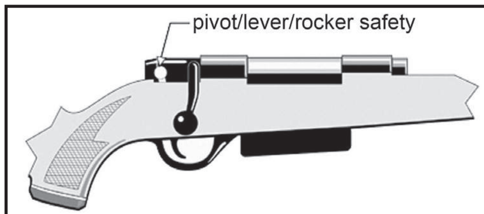
Figure 42. Pivot/Lever/Rocker Safety
