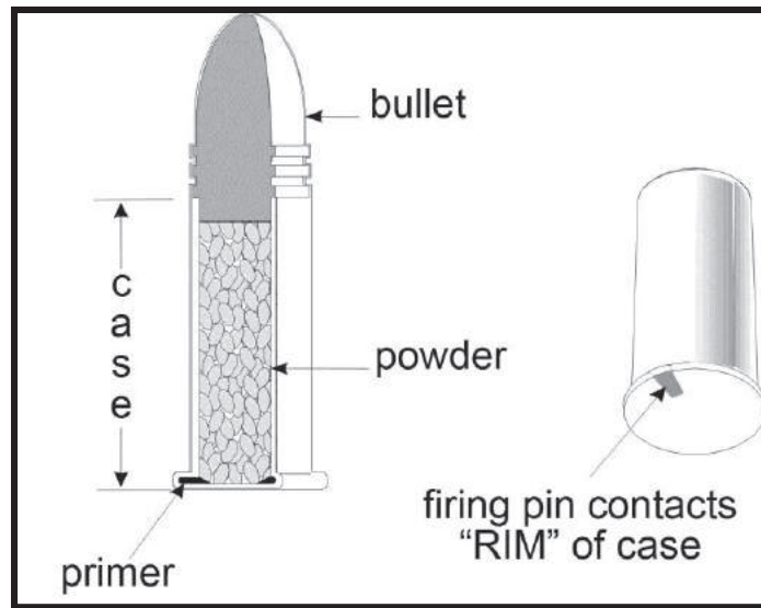
Figure 21. Rim-fire Cartridge
