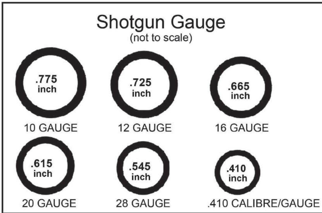
Figure 29. Shotgun Gauges
