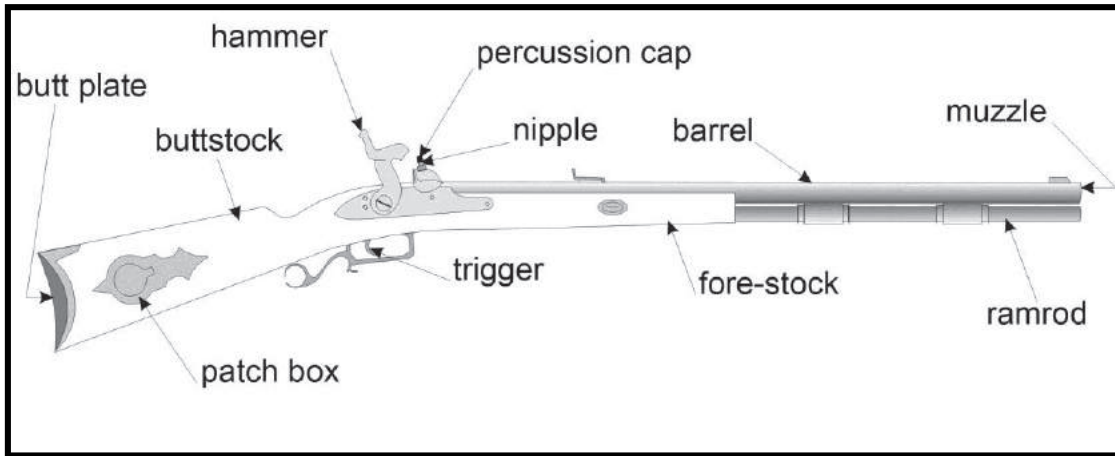
Figure 8. Muzzleloader
