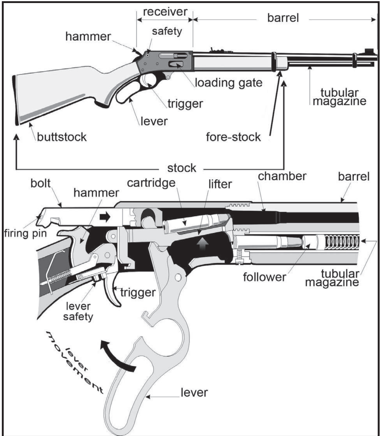
Figure 53. Lever Action
