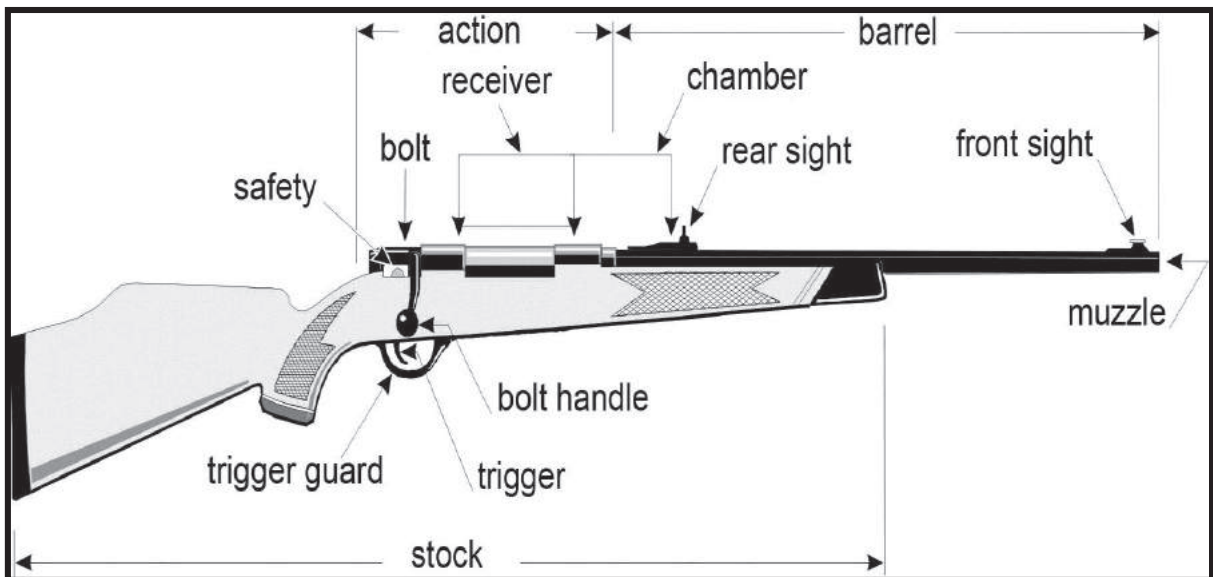
Figure 47. Bolt Action
