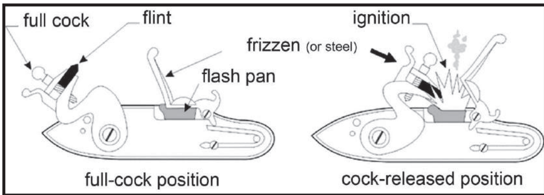
Figure 4. Flintlock Mechanism
