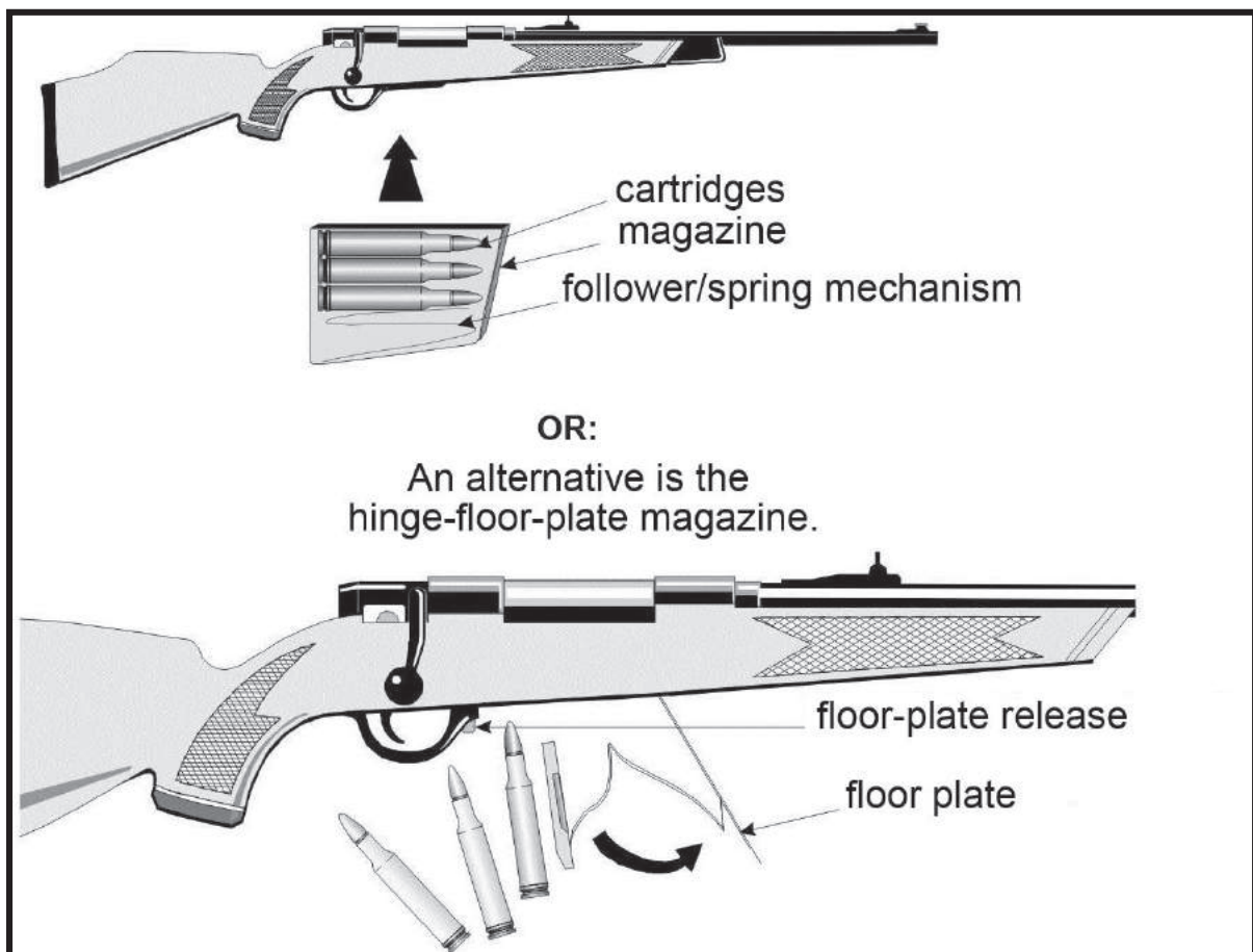
Figure 49. Box-type Magazine
