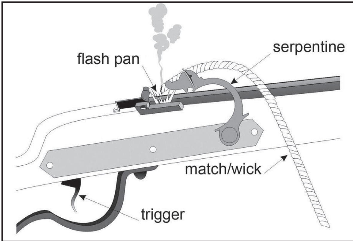
Figure 2. Matchlock Mechanism
